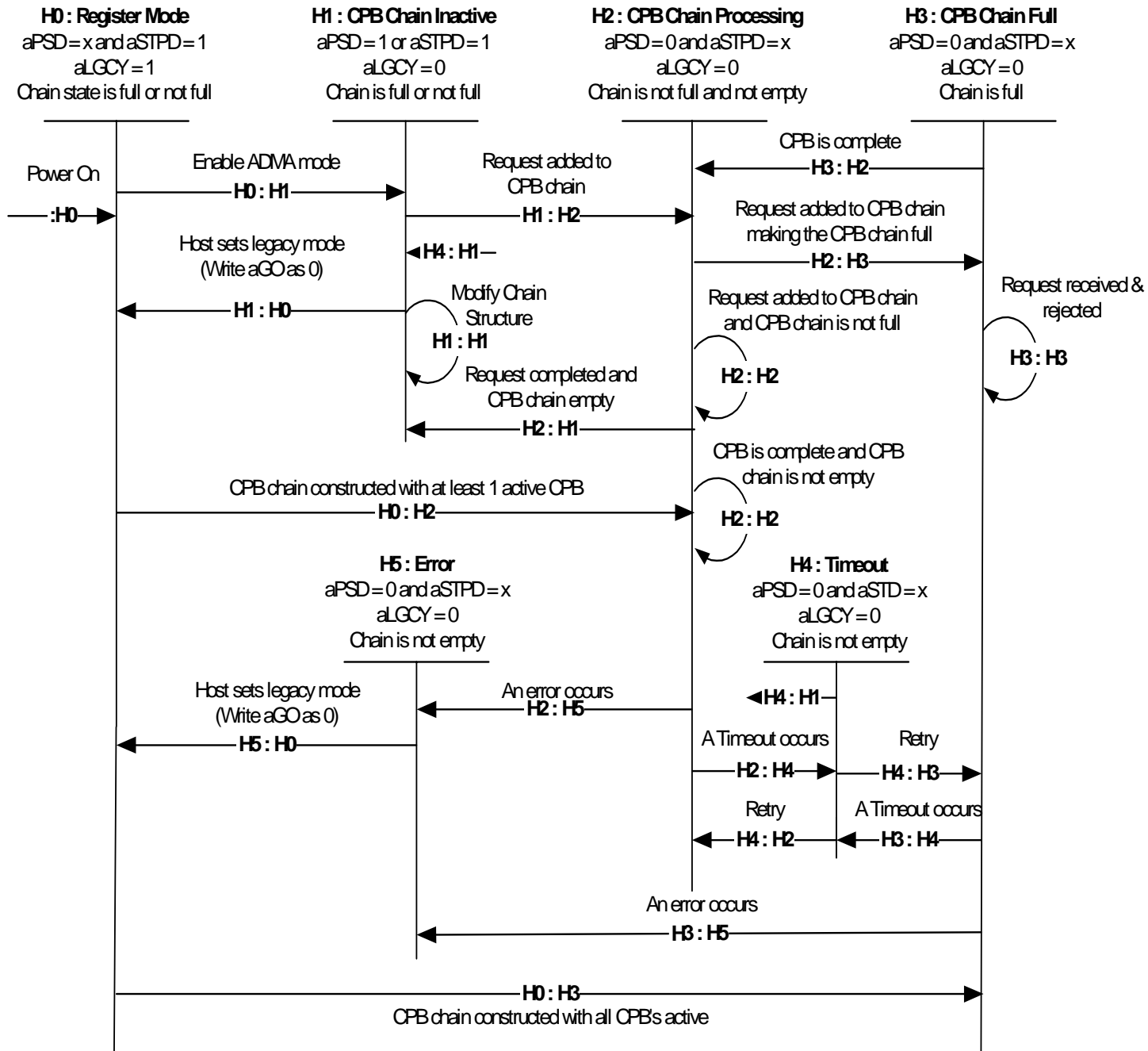
Figure 6 – Host Software States
