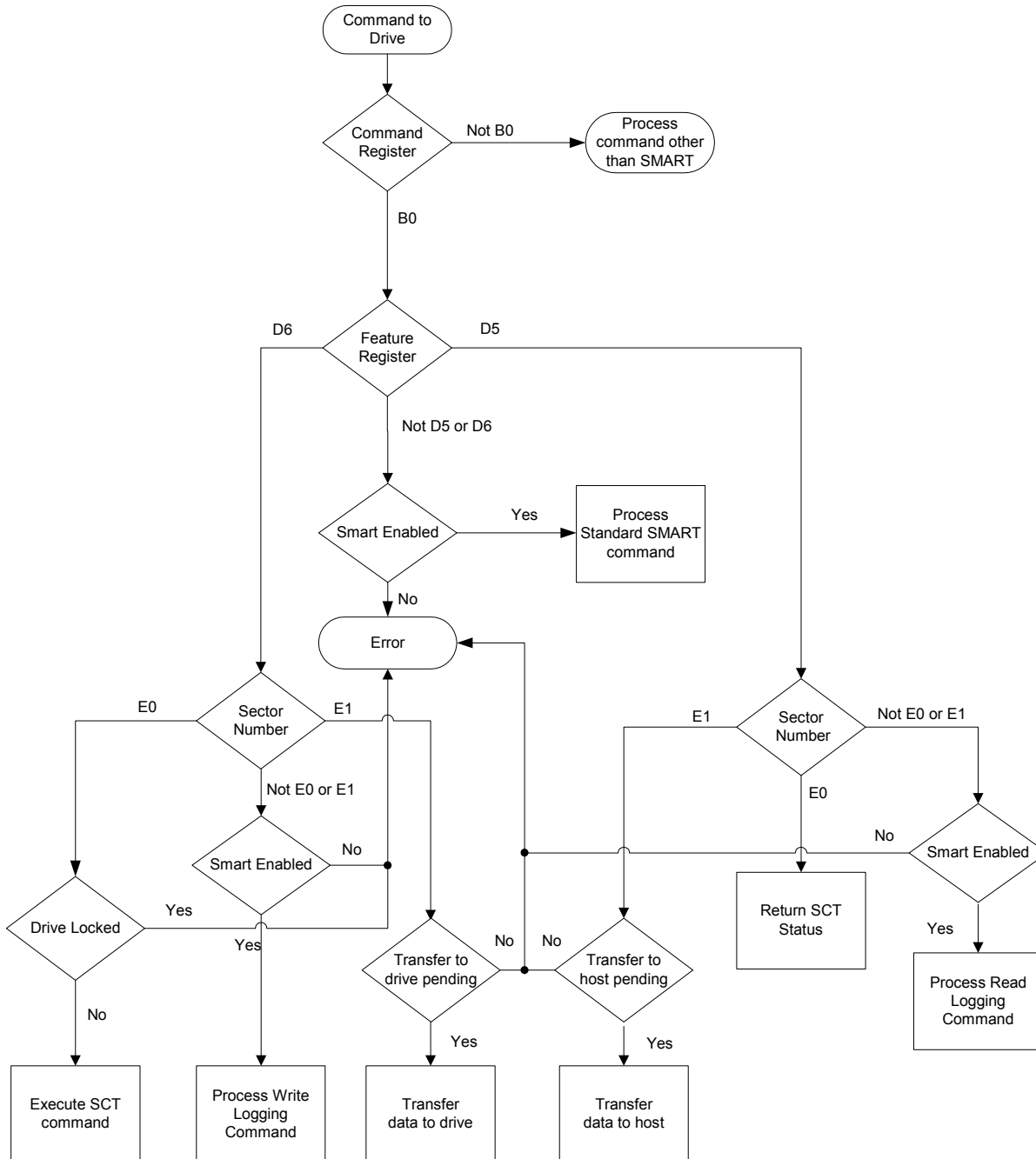
Figure 1– Command Decode
