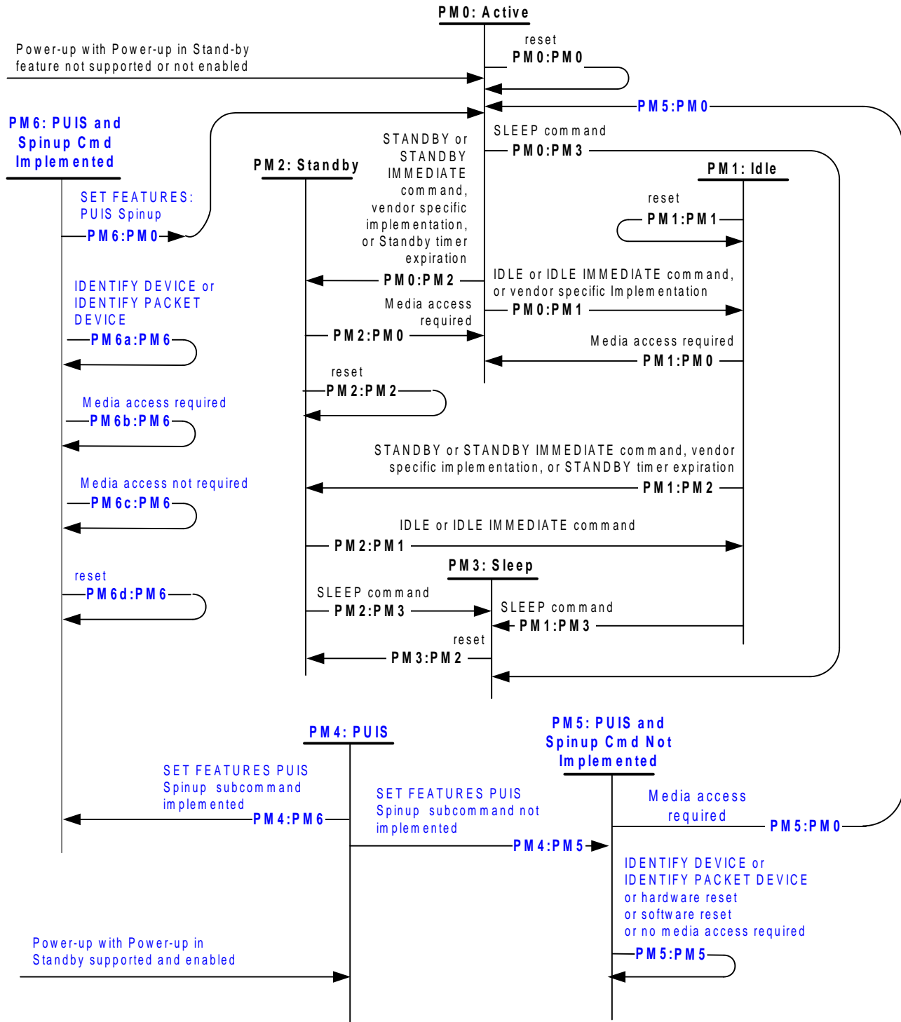
Figure 1 — Power Management State Diagram
